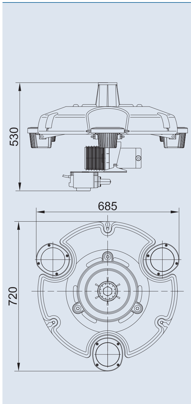
1"-thread with nozzle Here, as an example with a mounted Schaumsprudler 35-10E.
